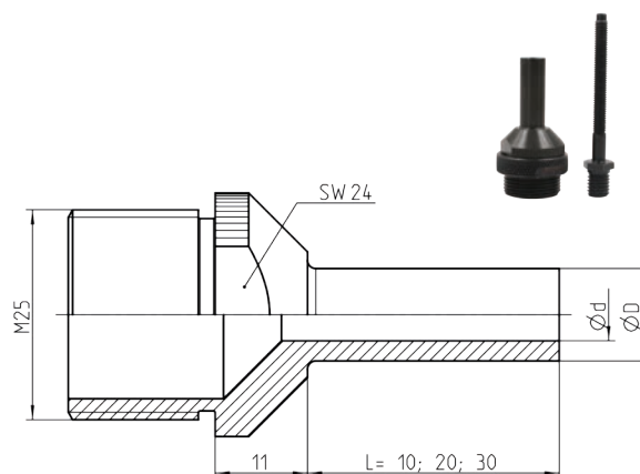
SL nosepiece FireBird® Pro/FireFox®
