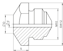
Special version 17/.....MB Nosepieces
